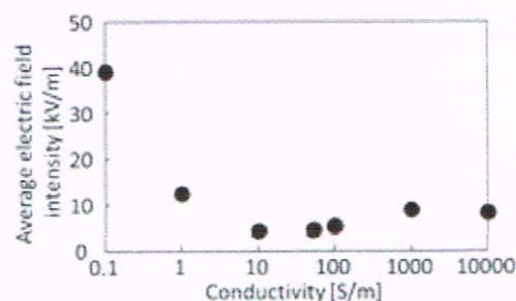
Fig. 2 Average electric field intensity in the cavity space as a function of the electrical conductivity of the CHT.
