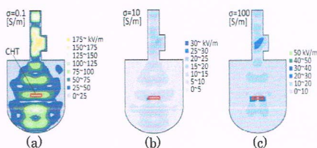
Fig. 1 Calculated cross-sectional electric field distributions in cavity (a) 0.1 S/m CHT, (b) 10 S/m CHT (c) 100 S/m CHT when the microwave of 200W output.
